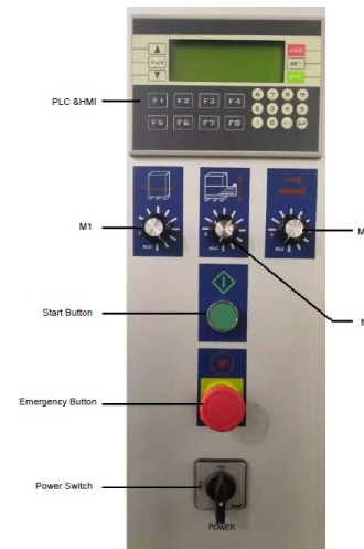
Control Panel
